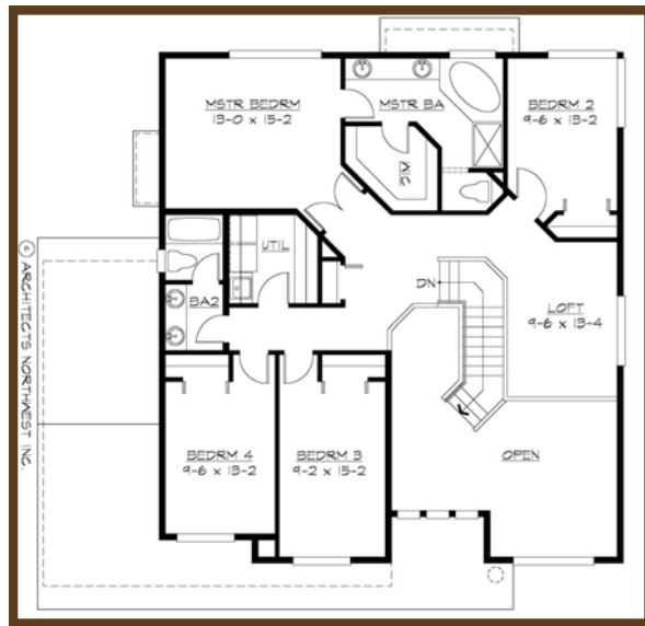
Upper Floor
